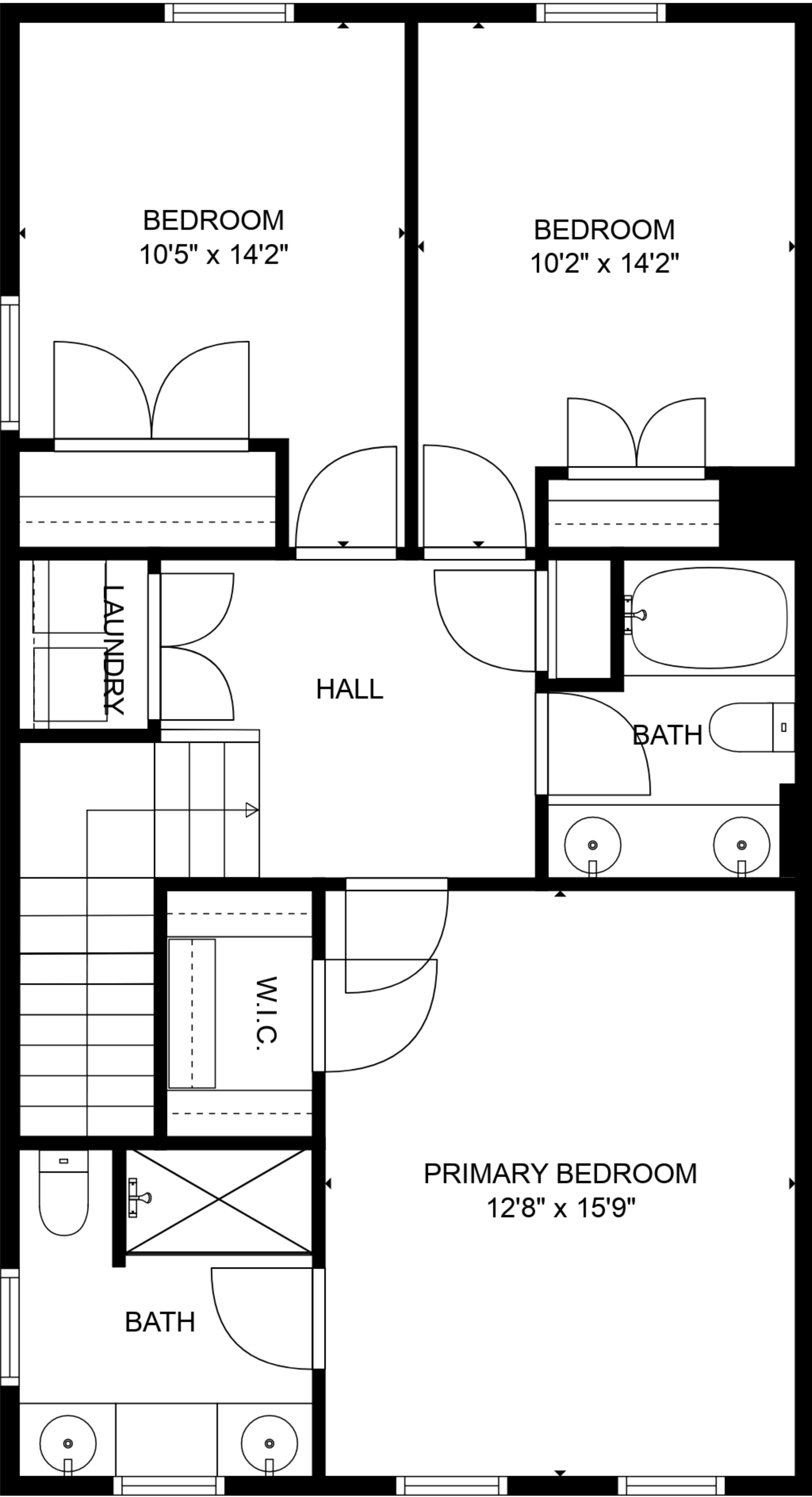
FLOOR 3
